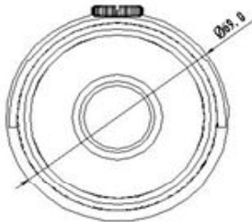
Contour dimension Unit: mm
